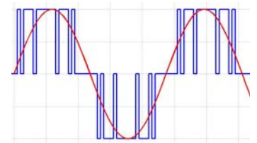
PWM in blue, SINUS in red
